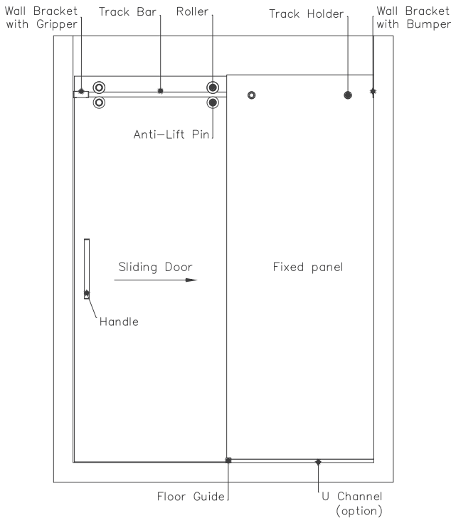
Layout 1-2 One fixed panel and one sliding glass door with a towel bar and a flush pull or a shower handle
