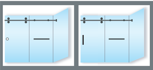
Layout 2-2 Sliding Door, Fixed Panel and 90° Return Panel with a towel bar and a flush pull or a shower handle
