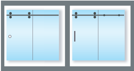
Layout 1-1 One fixed panel and one sliding glass door with a flush pull or a shower handle
