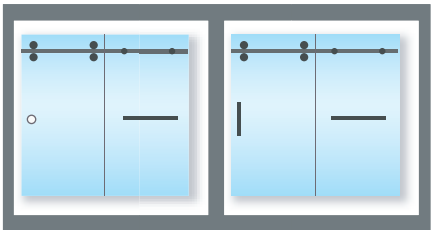
Layout 1-2 One fixed panel and one sliding glass door with a towel bar and a flush pull or a shower handle
